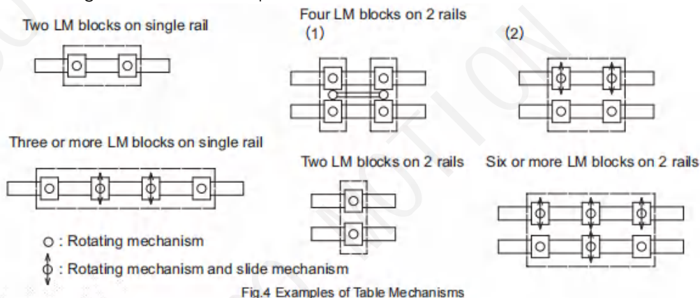
Fig.4 Examples of Table Mechanisms
