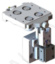
Lifting and positioning mechanism
