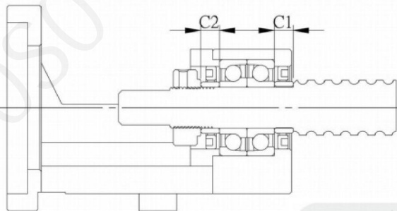
Rolled Ballscrew
