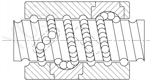
Fig 1.6.1 U,I,M-Type Nut
