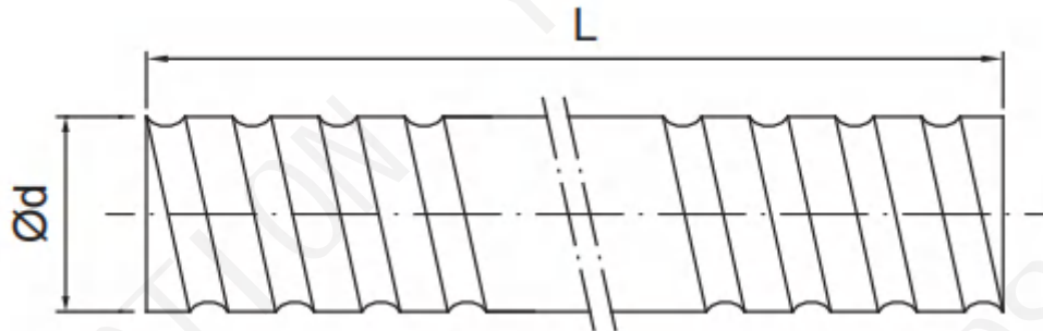
Fig 2.3.1 Screw Shaft Nominal Diameter
