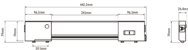
PL442S-SCREW FIX
